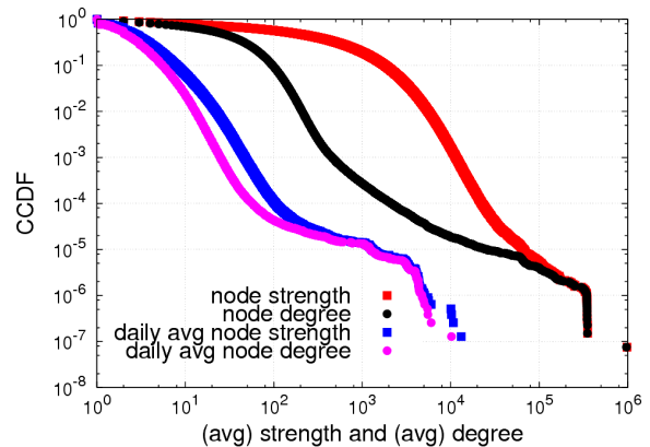
Figure 5: CCDF of strength and degrees of the activity network
