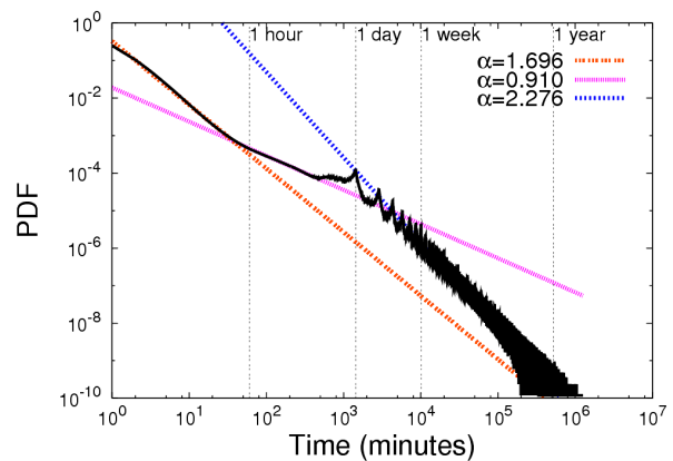
Figure 15: Time intervals between guestbook comments
